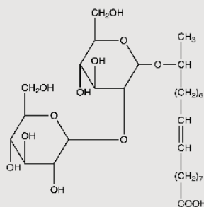
Acidic sophorolipid
