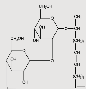
Lactonic sophorolipid
